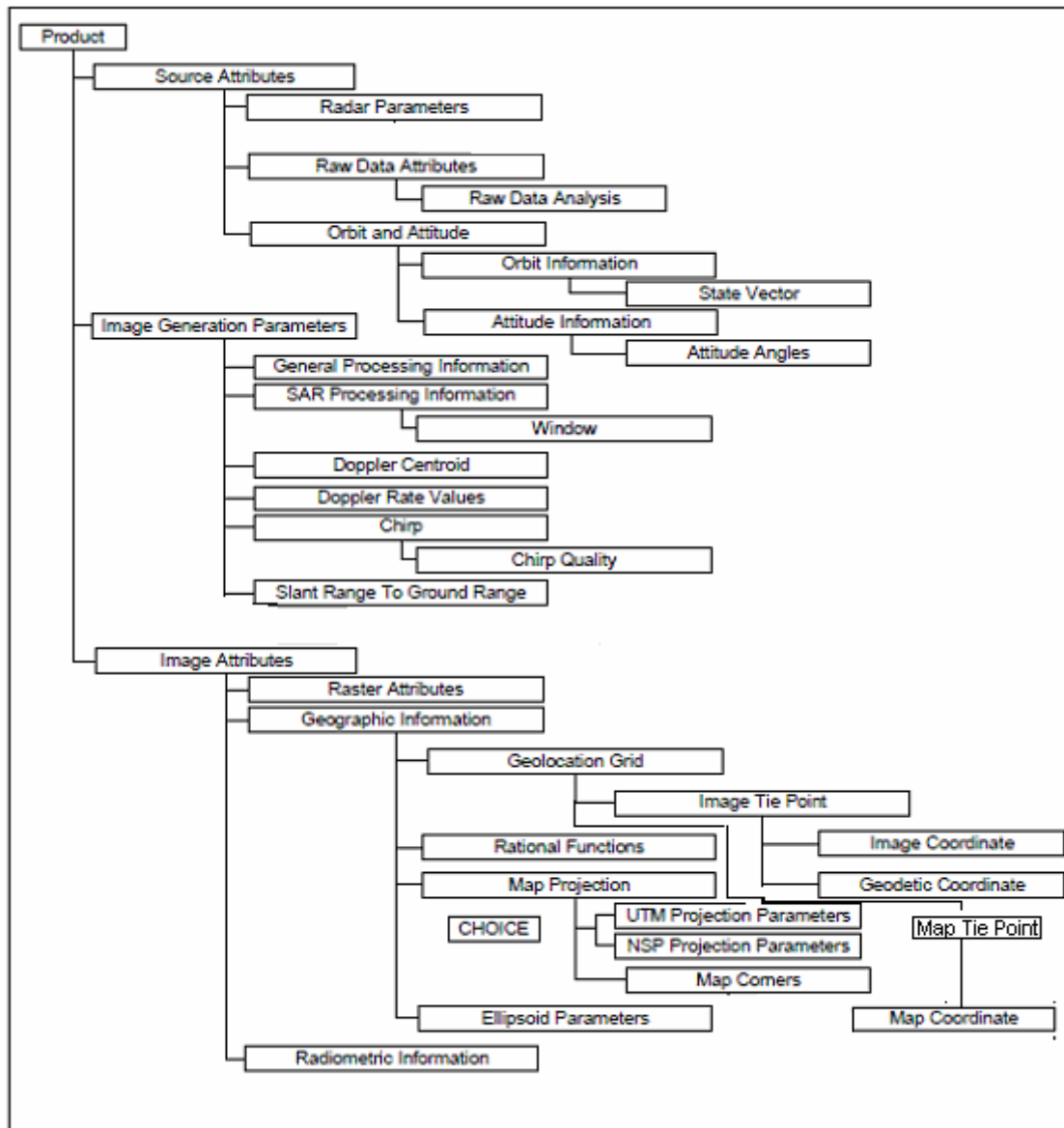
Fig A3.1 EOS-04 Product Hierarchy
